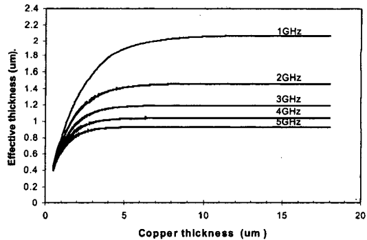
Fig.3 Effective copper thickness for different frequency
