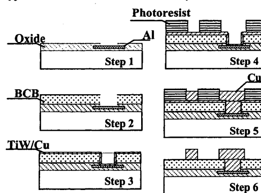
Fig.1. Process flow and cross-sectional schematic of the high-Q inductors: Step 1): oxide and metal one (aluminum) patterning; 2) BCB coating and via opening; 3) TiW/Cu seed
